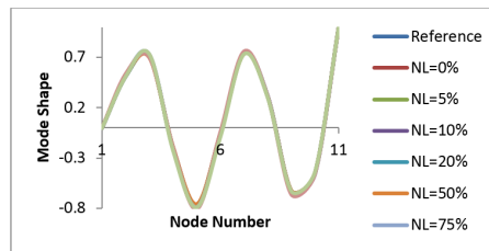
Figure 8: The fifth mode shape of beam CF
