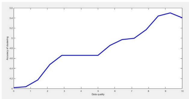
Figure 19: Check data quality and clustering accuracy
