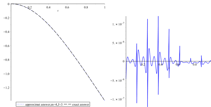
Figure 4: The numerical solution of Example 5.2 for m = 4, J = 3 and the exact answer and error values
