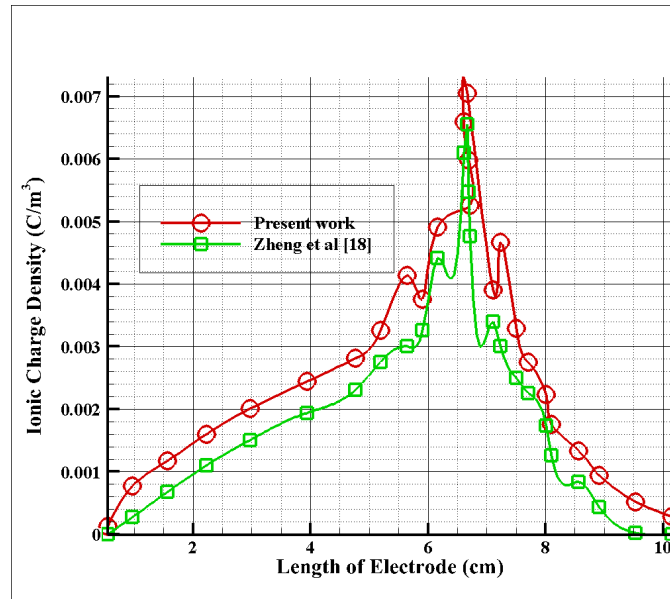
Figure 2: Comparison of the ion density diagram of the current work with the work of Zheng et al. [1]
