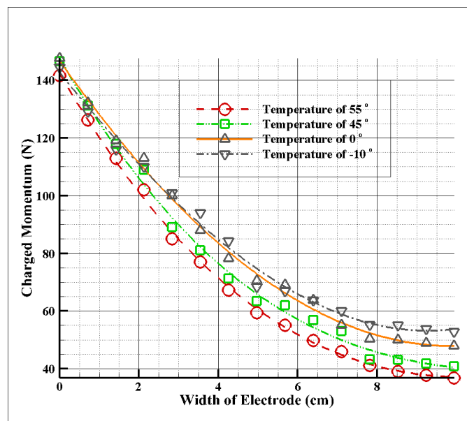
Figure 7: Momentum changes due to ion charge in the distance between two electrodes according to different temperatures at a pressure of 8.0 bar
