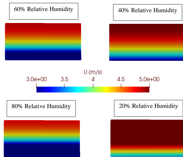
Figure 4: Speed contour according to the types of relative humidities studied in this research at a pressure of 4.0 bar, the higher the speed value is in the higher range, the higher the momentum is transmitted
