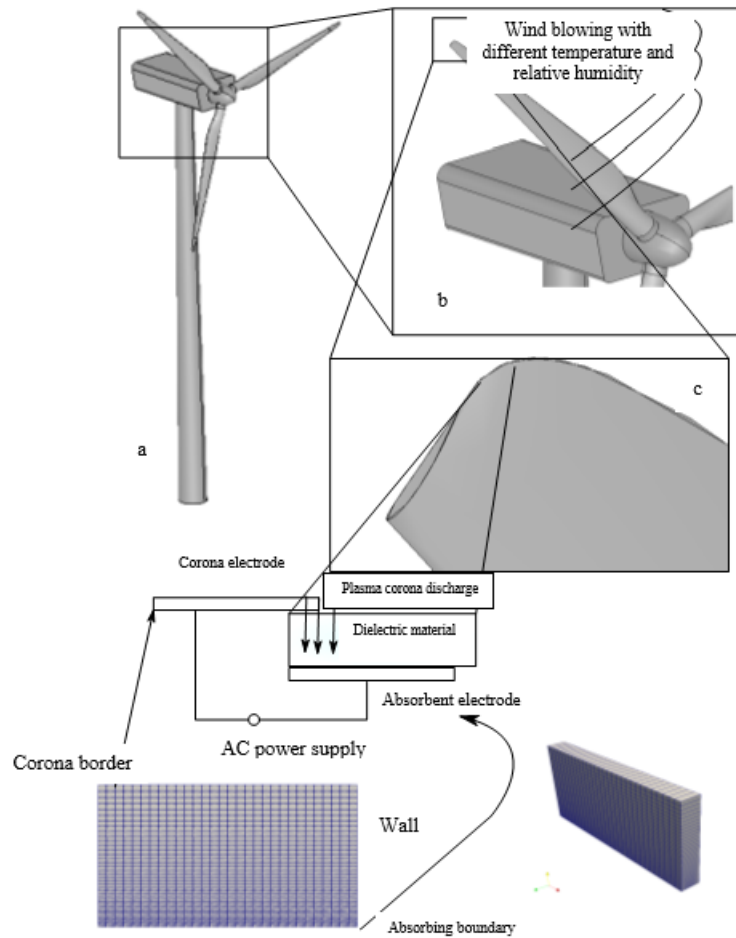
Figure 1: Different views of the wind turbine blade geometry, and the grid around the considered airfoil
