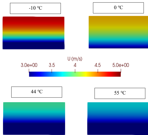
Figure 6: Speed contour according to the types of temperatures studied in this research at 8.0 bar pressure, the higher the speed value is in the higher range, the higher the momentum is transmitted
