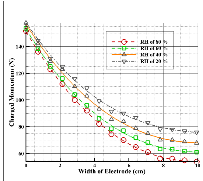
Figure 5: Momentum changes due to ionic charge in the distance between two electrodes according to types of relative humidities at 4.0 bar pressure
