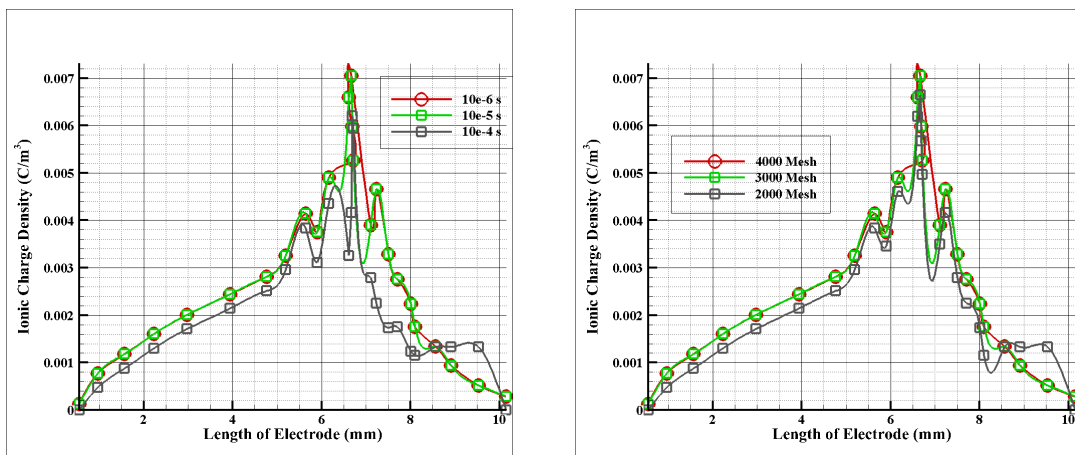
Figure 3: Right side: independence of results from meshing and left side independence of results from time step
