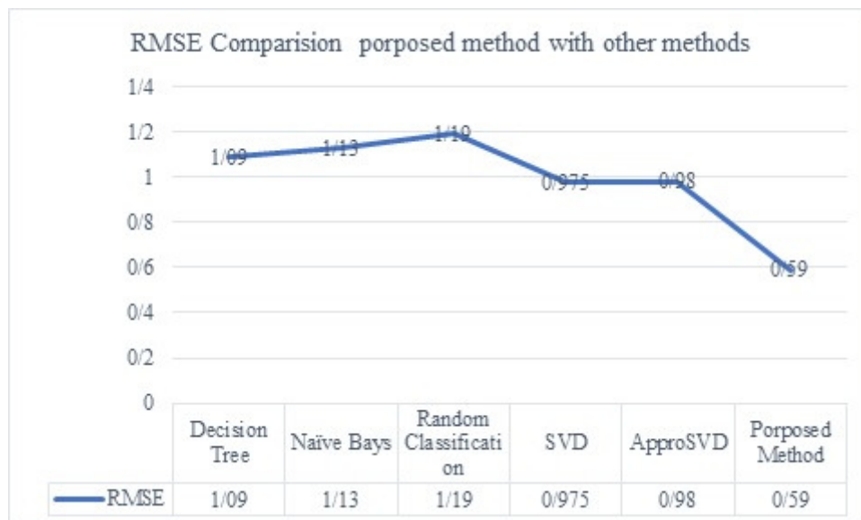
Figure 9: RMSE Comparison.
