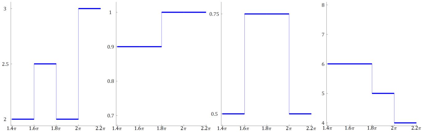
Figure 3: The best efficient staircase-function strategies producing payoffs (10.8) in the 0.2\pi -extended 4-person staircase-function game (5.7) by (10.3)—(10.6) and (10.1)
