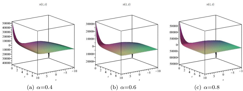
Figure 2: Numerical simulation of the power series solution (5.13) with p = 3, C_1 = C_2 = C_3 = 1, a_0 = a_1 = a_2 = 1 and s = x + y + z .
