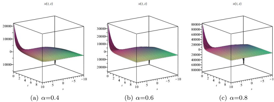
Figure 1: Numerical simulation of the power series solution (5.13) with p = 2, C_1 = C_2 = C_3 = 1, a_0 = a_1 = a_2 = 1 and s = x + y + z .
