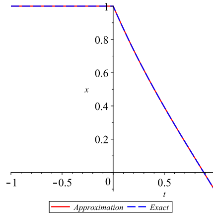
Figure 1: Approximation and exact values of state variable for Example 4.1
