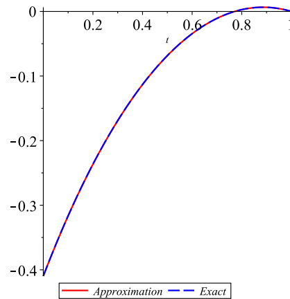
Figure 2: Approximation and exact values of control variable for Example 4.1
