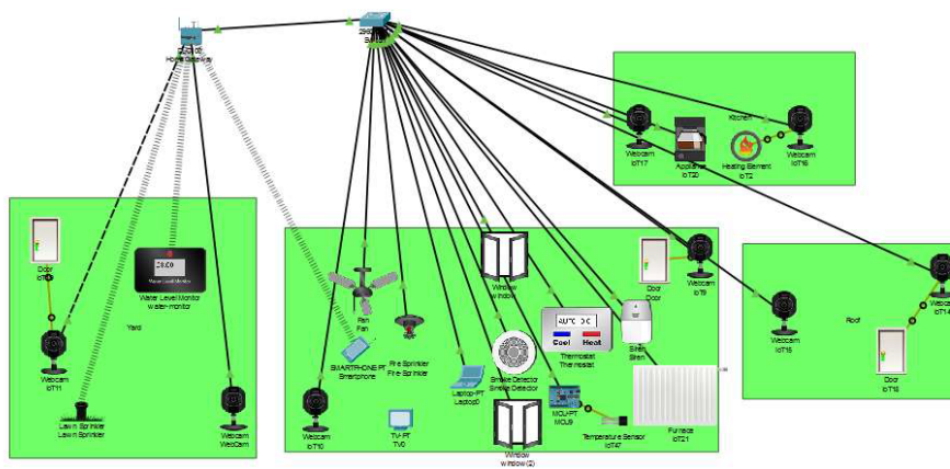
Figure 1: Presented Model
