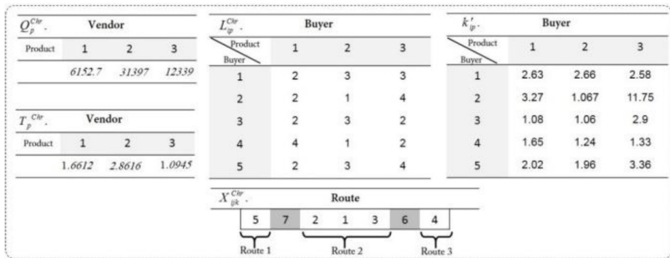
Figure 2: Chromosome Structure of Presented Model
