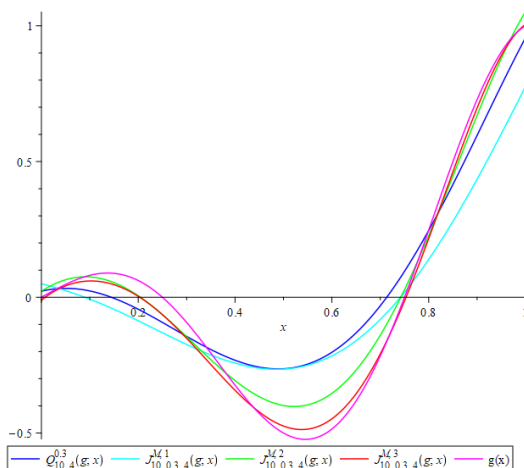
Figure 3: Approximation process
