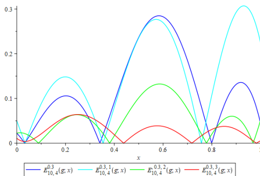
Figure 4: Error estimation
